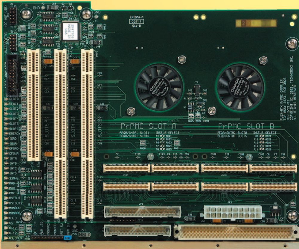
3923 PrPMC Carrier
