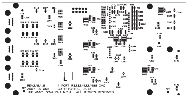
Component Placement View - Side 2
