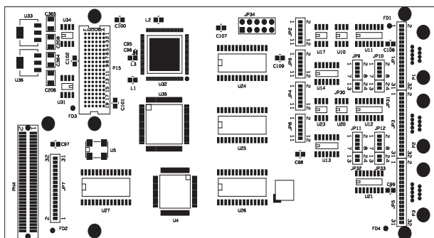
Component Placement View - Side 1
